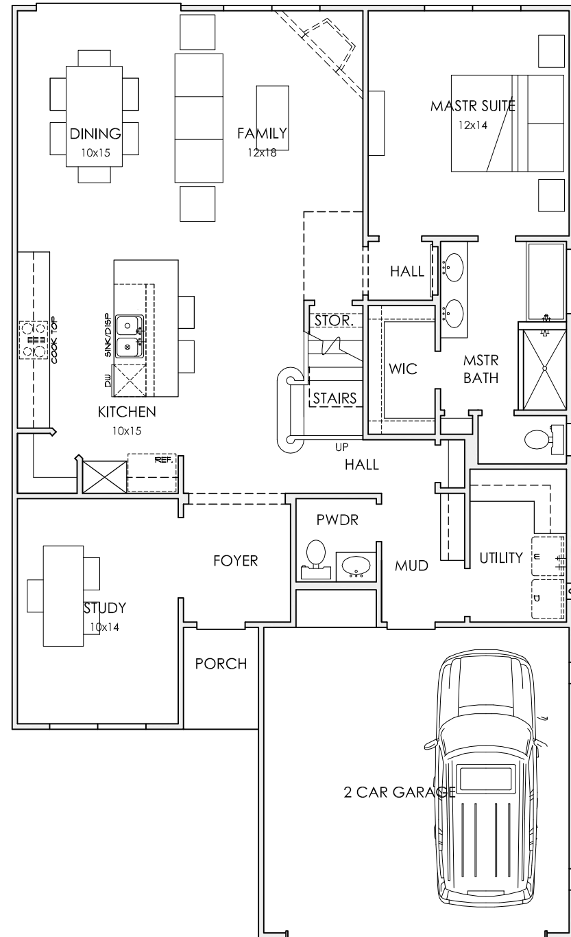
1st FLOOR PLAN 1,409 sq. ft.
